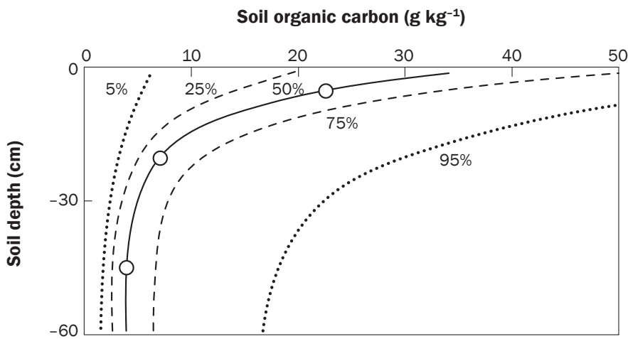
Figure 3 Statistical limits of soil organic carbon distribution by depth across 310 fields in North Carolina.
